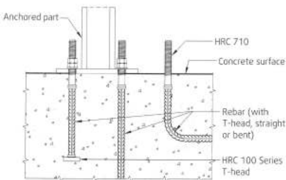
Fig. 4 Illustrations of HRC 710 used for mechanical fastening of a steel structure, including different variants of the reinforcement bar
