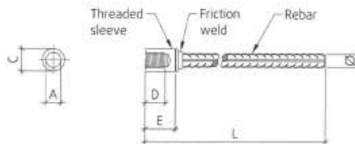
Fig. 2 Geometry HRC 720 / HRC 720SS, see Table 2
