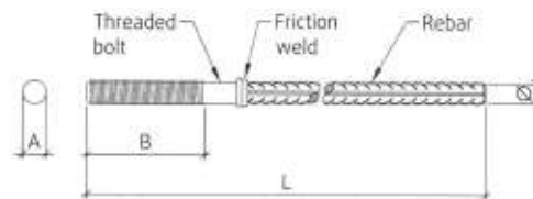
Fig. 1 Geometry HRC 710, see Table 1
